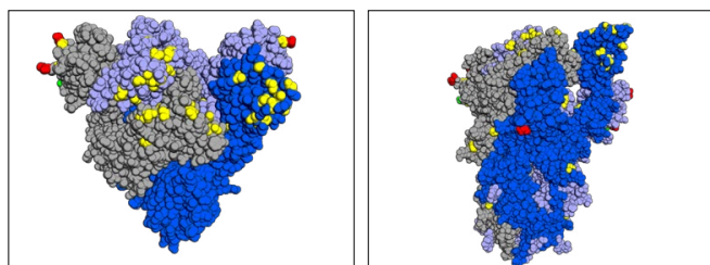
Figure 2: Illustration of the locations of the Omicron mutations in the spike protein, top Left picture and right picture, showing amino acid substitutions which has shown in color yellow, deletions (red), and insertions (green). In this trimeric structure, two monomers (gray and light blue) have their receptor-binding domains in the down conformation while one (dark blue) is in the up or open conformation. Mutation data from WHO, structure from PDB: 6VYB.
